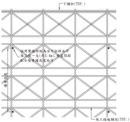
(P)繫牆桿配置圖
