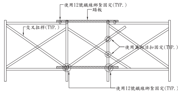
SEC M-M
